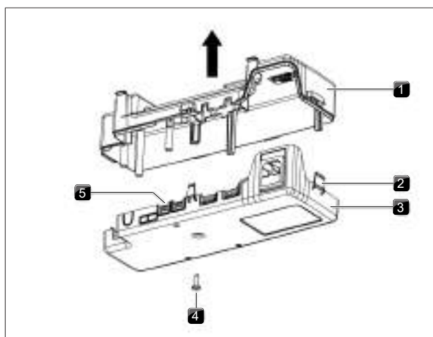
Fig. 4.59 Opening the control unit housing cover
