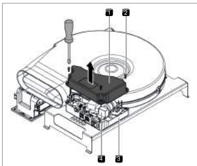
Fig. 4.58 Opening the control unit housing cover
