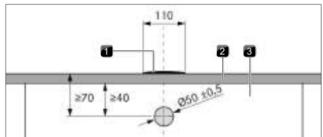
Fig. 4.16 Cooktop extractor drilling pattern
